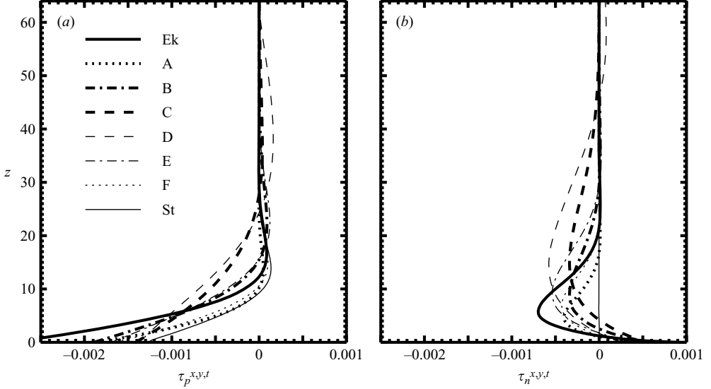
FIGURE 7. As figure 6, but for the time-averaged stresses, (a) \bar{\tau}_p^{x,y,t} and (b) \bar{\tau}_n^{x,y,t} .
