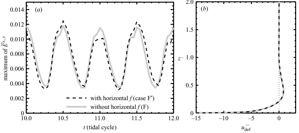
FIGURE 15. (a) Time evolution of the maximum value of \overline{E}^{x,y} and (b) the vertical profile of the time-averaged velocity defects, \overline{u}_{\text{def}}^{-x,y,t} . Grey solid (black dashed) lines indicate case F (case F').
